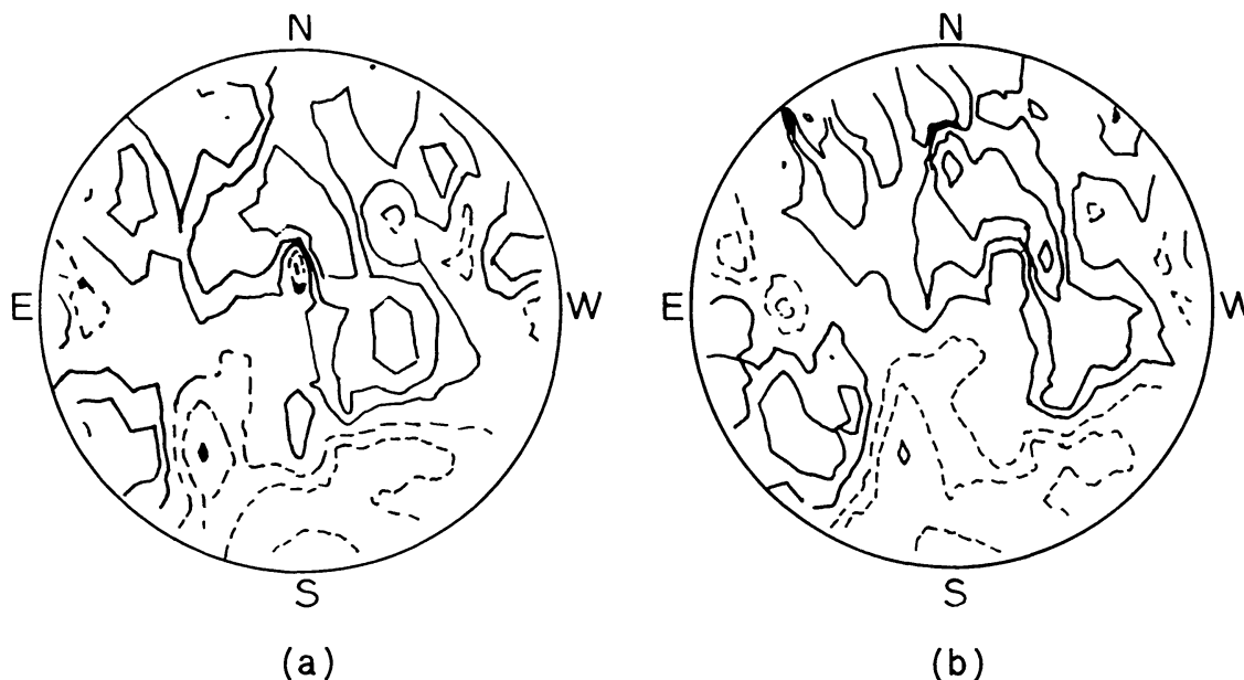
Fig. 2. Magnetograms made at Stanford with 3' resolution ( \approx 1/10 of the solar diameter). The spectral line used is Fe I \lambda 5250.2 Å. The statistical error is approximately 0.05 G for each datapoint. The contour levels shown are \pm 0.2 , \pm 0.5 , \pm 1.0 , \pm 2.0 G. (a) May 5, 1976. (b) May 6, 1976.
